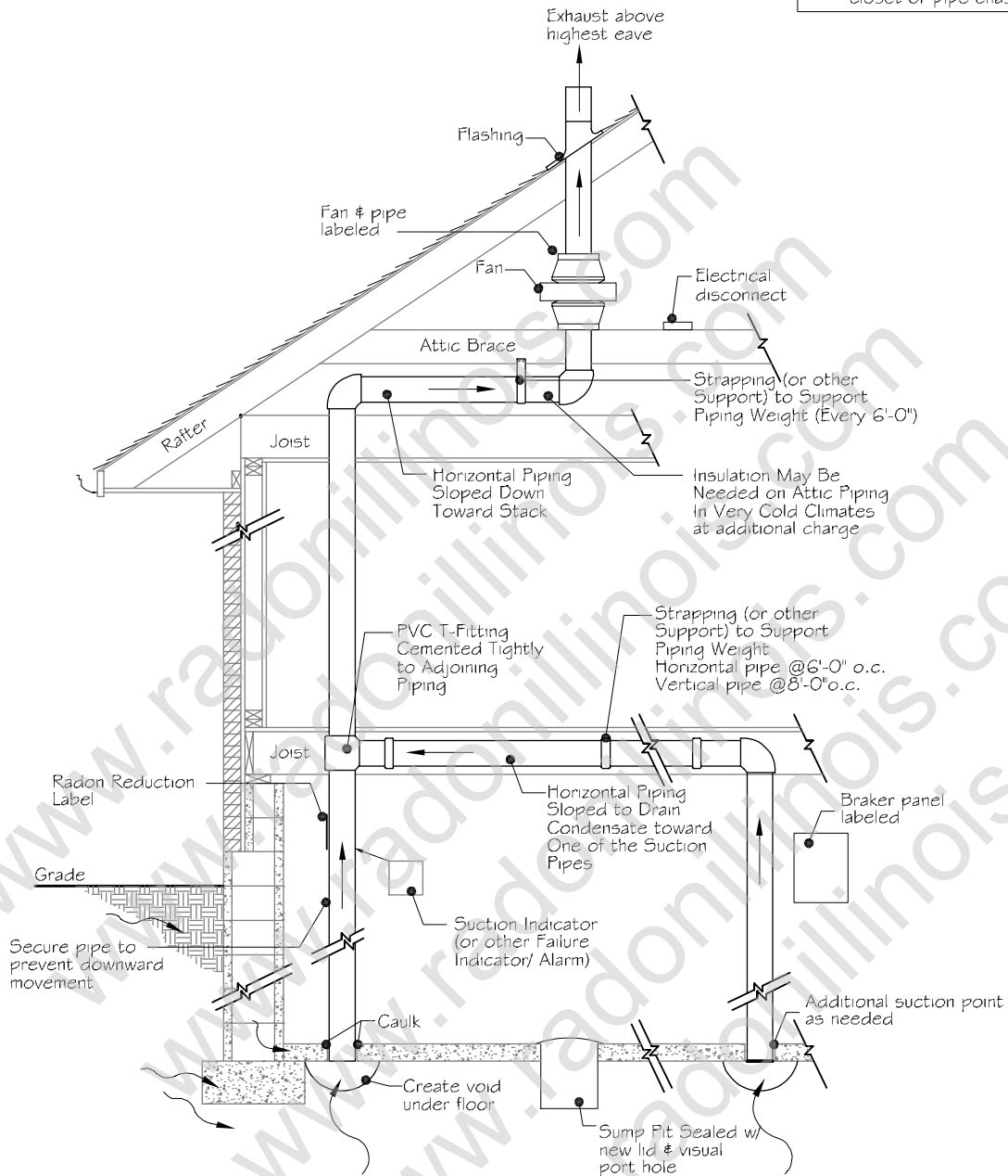
RADON MITIGATION SYSTEM CONFIGURATION illustrating an interior exhaust stack
