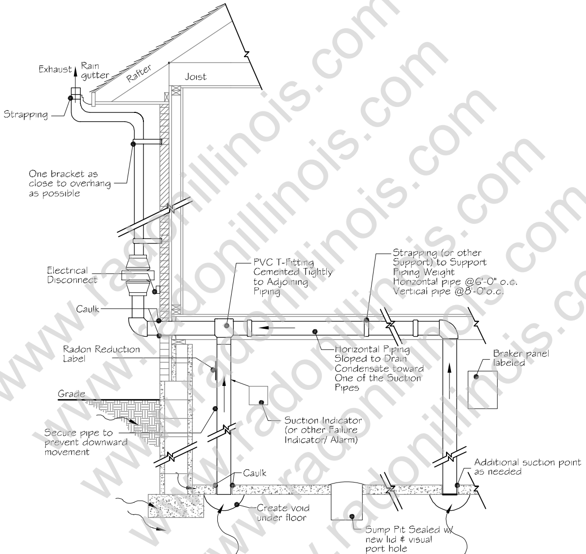
RADON MITIGATION SYSTEM CONFIGURATION Illustrating an exterior exhaust stack
